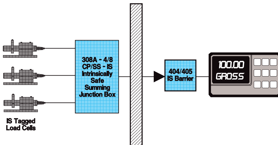
Figure 7. Division 1 and ordinary location application: intrinsic safety barriers required; instrument located in safe area.
