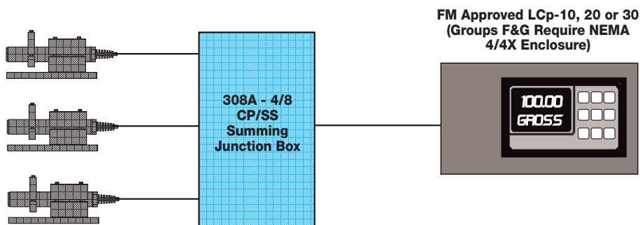
Figure 6. Division 2 application: non-incendive; intrinsic safety barriers not required.
